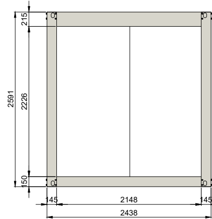
Facade "B"
