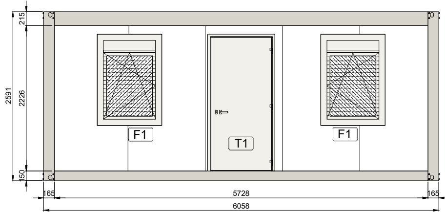
Facade "A"
