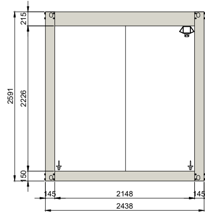
Facade "D"
