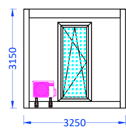
View "C"
